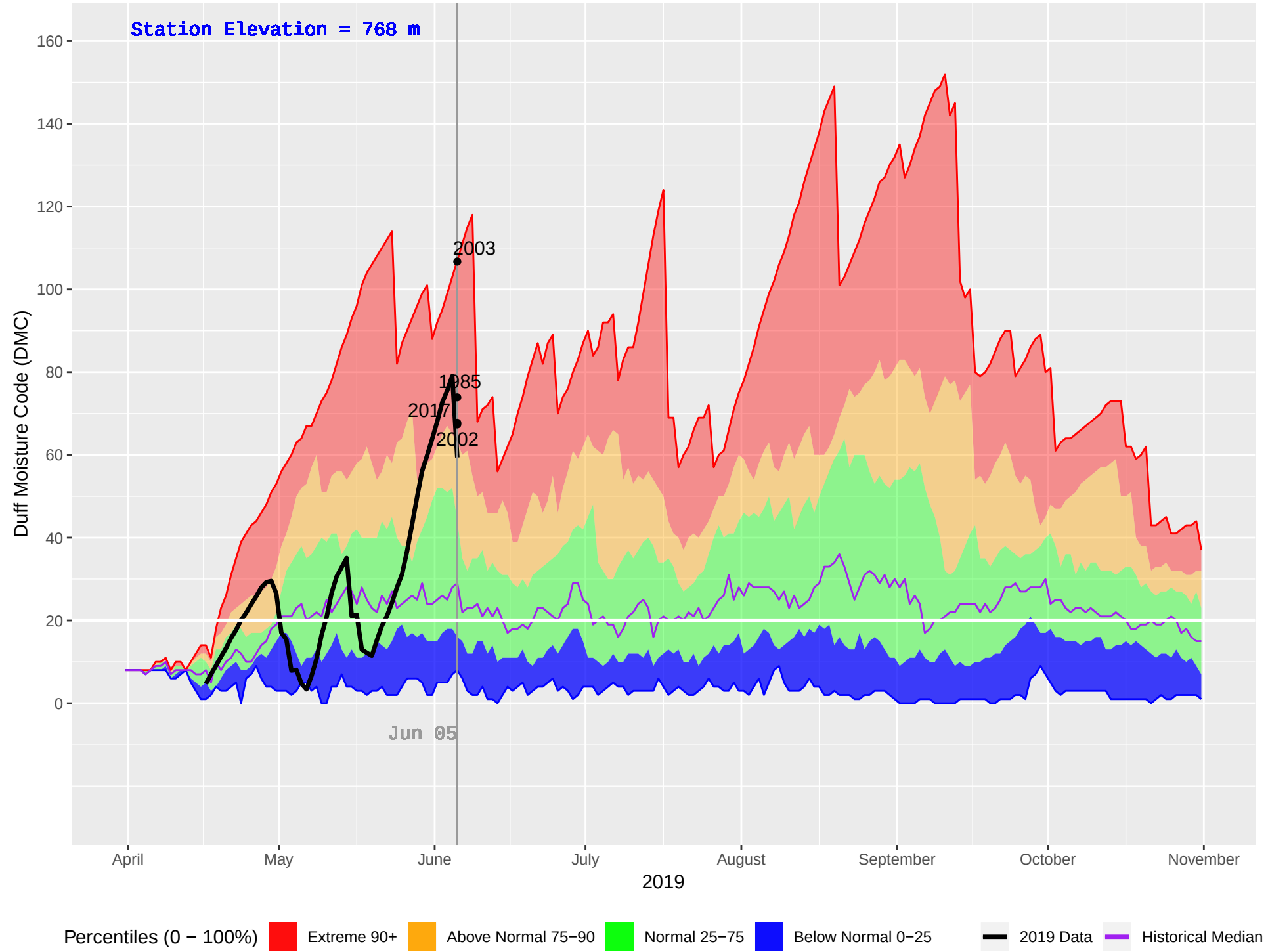
GRAHAM (124) : Historical (1979–2018), Current (2019) Daily Duff Moisture Code (DMC)
