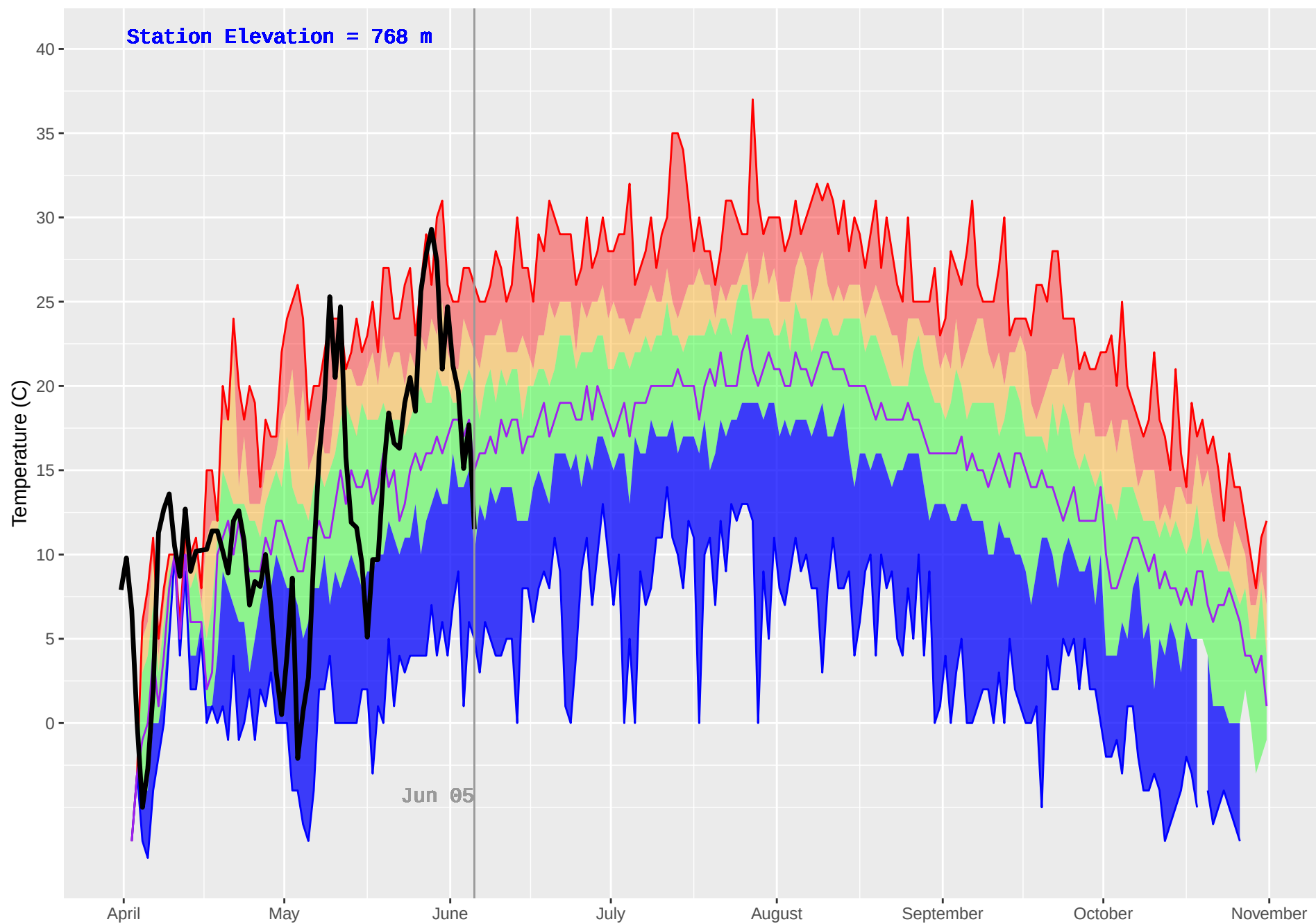
GRAHAM (124) : Historical (1979–2018) and Current (2019) Daily Temperature
