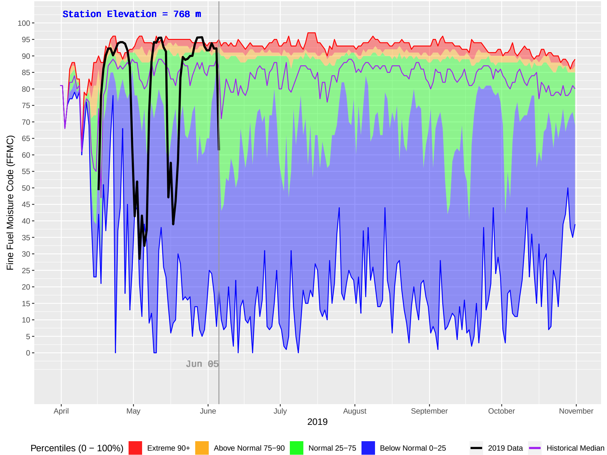
GRAHAM (124) : Historical (1979–2018) and Current (2019) Daily Fine Fuel Moisture Code (FFMC)
