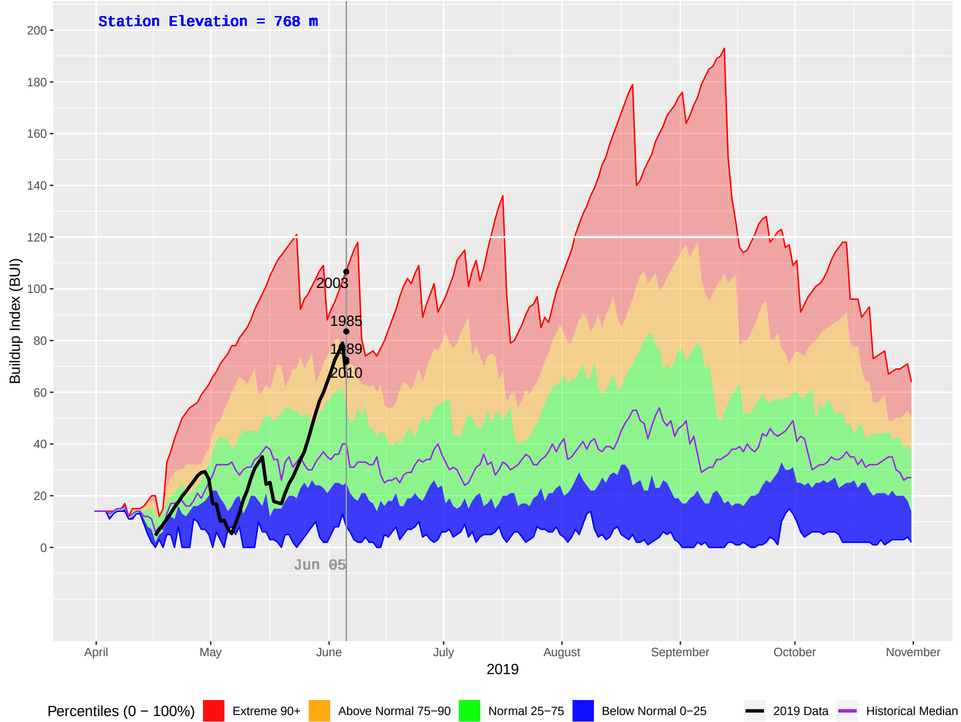
GRAHAM (124) : Historical (1979–2018), Current (2019) Daily Buildup Index (BUI)
