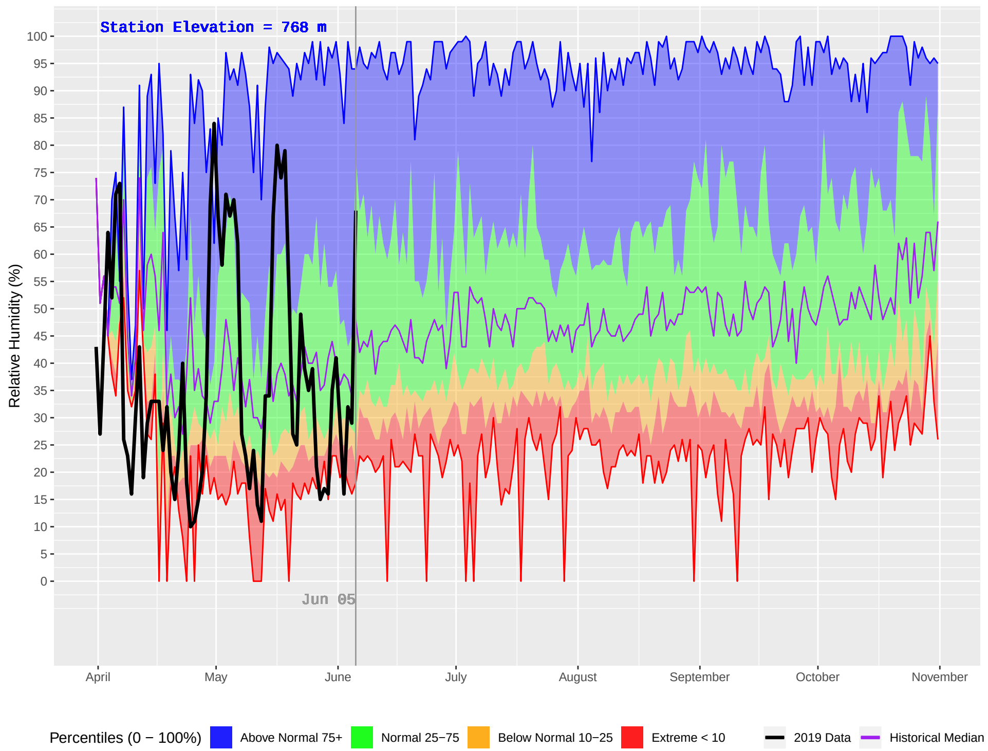
GRAHAM (124) : Historical (1979–2018) and Current (2019) Daily Relative Humidity
