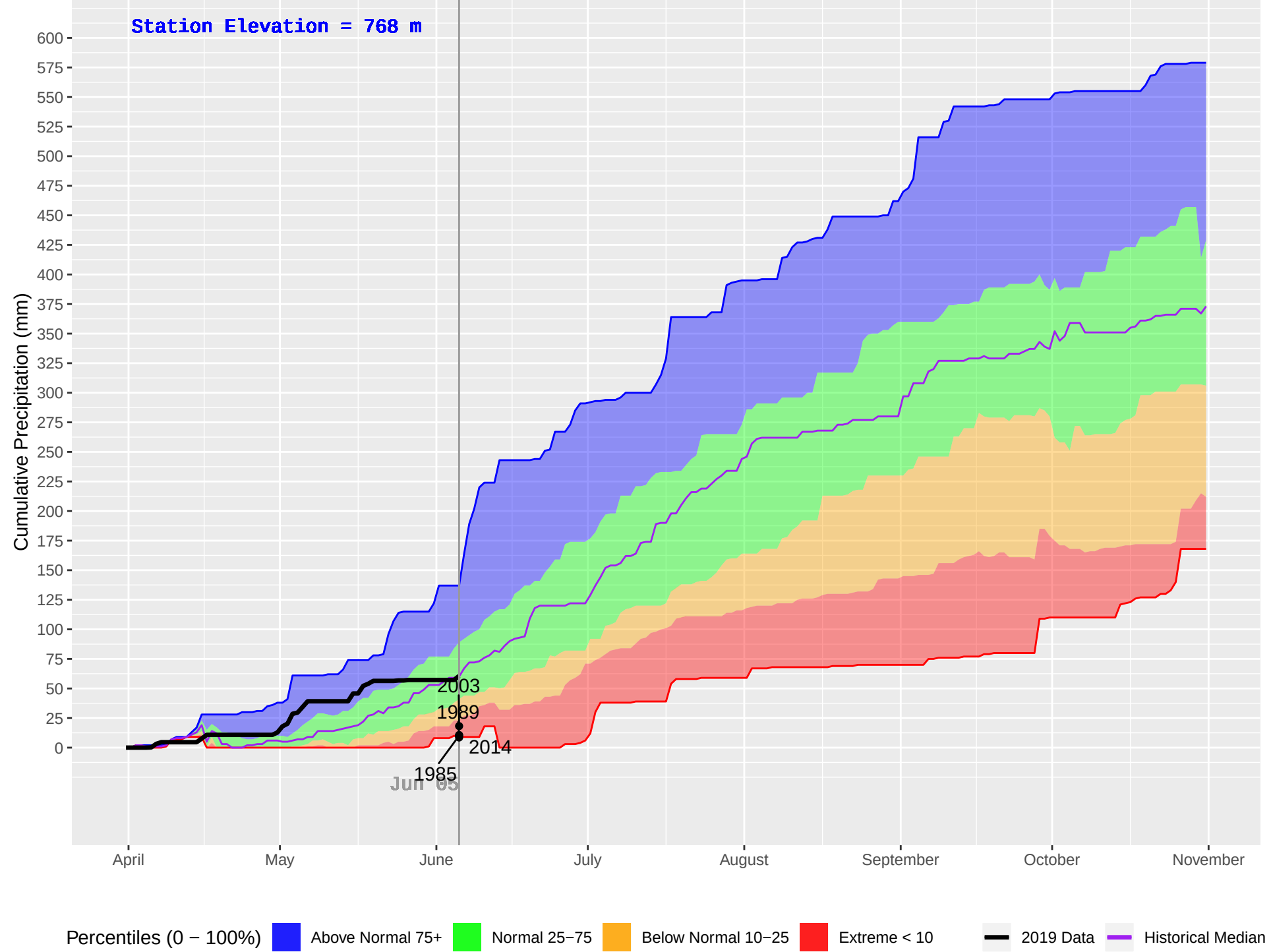
GRAHAM (124) : Historical (1979–2018), Current (2019) Daily Cumulative Precipitation
