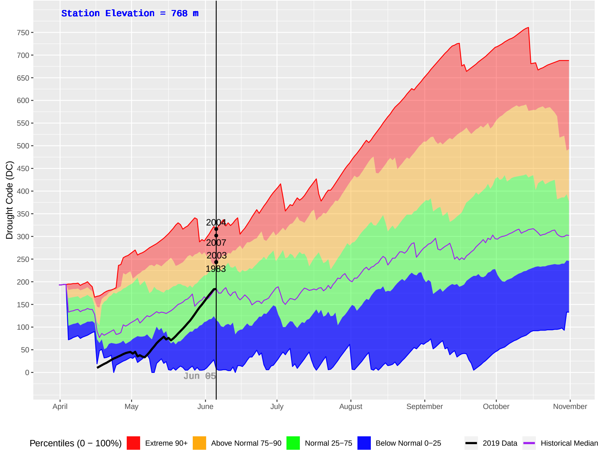
GRAHAM (124) : Historical (1979–2018) and Current (2019) Daily Drought Code (DC)
